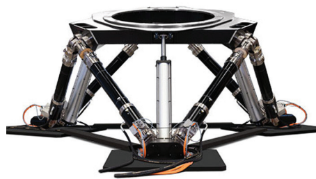
Turret Test System
