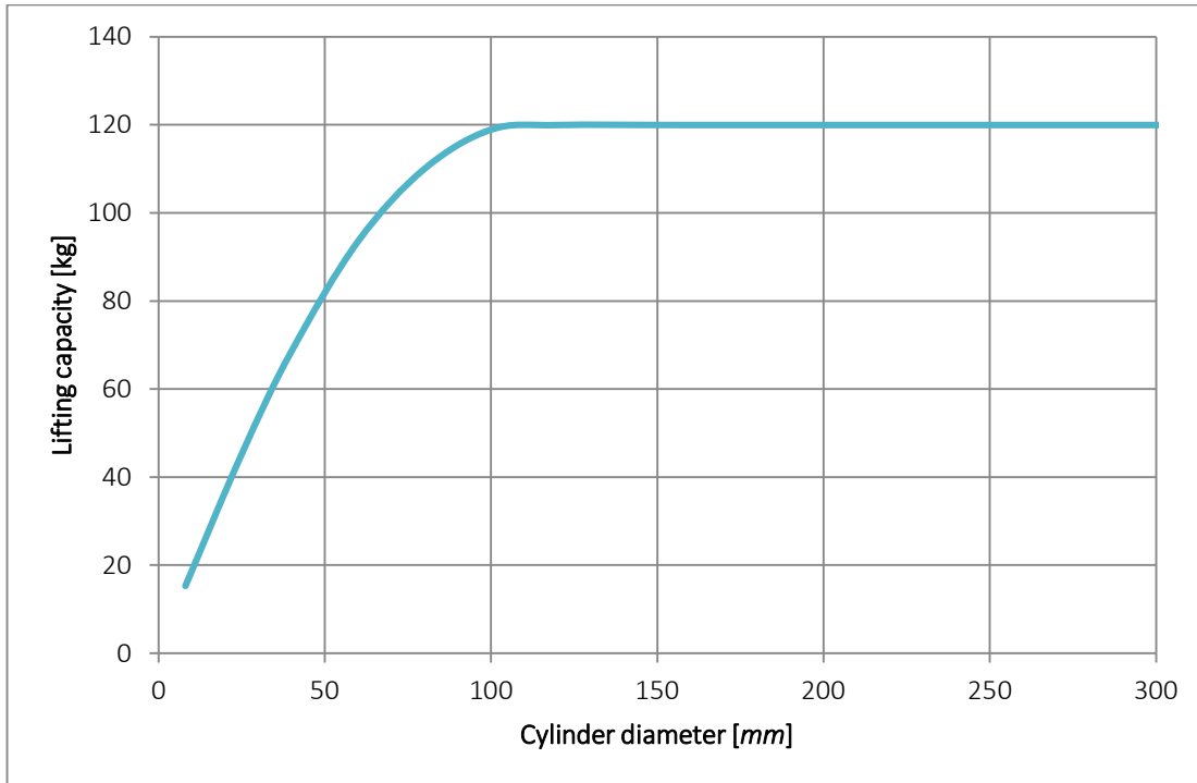
Figure 4. MRP-100NK lifting capacity in proportion to the diameter of a solid cylindrical part
