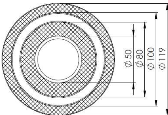
Figure 1. The gripping surface and magnetic poles of MAP-180.
