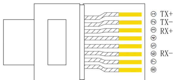
FIG 3 YDLIDAR TIA-H INTERFACES
