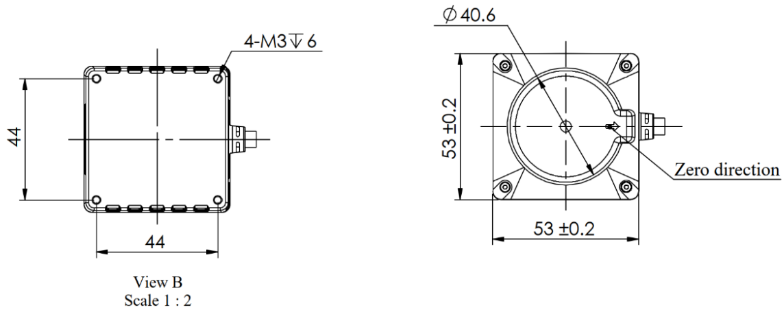
FIG 1 YDLIDAR TIA-H INSTALLATION DIMENSION (UNIT:MM)
