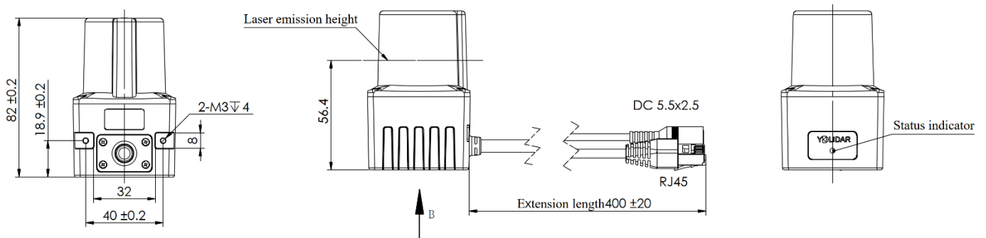
FIG 2 YDLIDAR TIA-H MECHANICAL DIMENSION (UNIT:MM)
