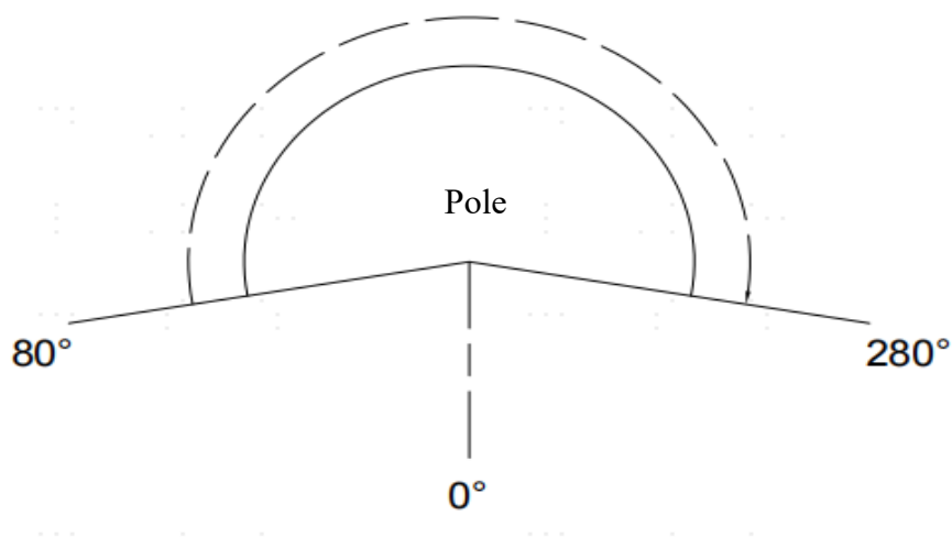
FIG 4 YDLIDAR TG5 POLAR COORDINATE SYSTEM DEFINITION
