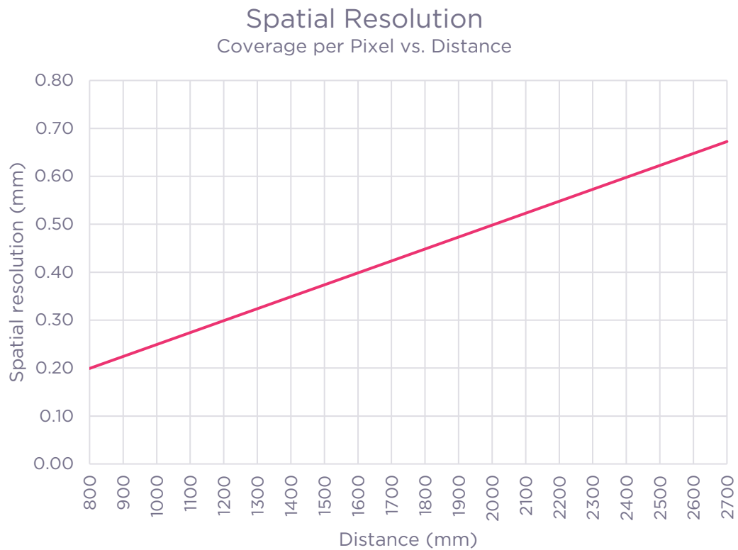
FIGURE 3 – SPATIAL RESOLUTION
