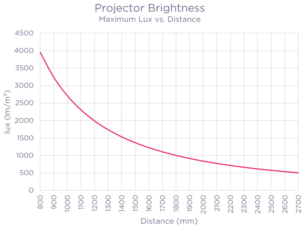
FIGURE 4 – PROJECTOR BRIGHTNESS
