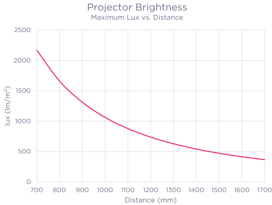
FIGURE 4 – PROJECTOR BRIGHTNESS
