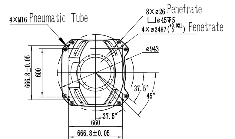
Base Installation Diagram
