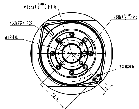
Base mounting holes
