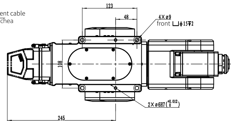
Base mounting holes
