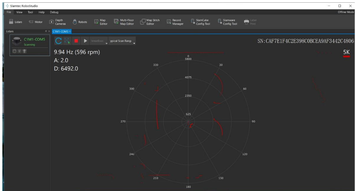
Figure 3-1 The Framgrabber Plugin in RoboStudio
