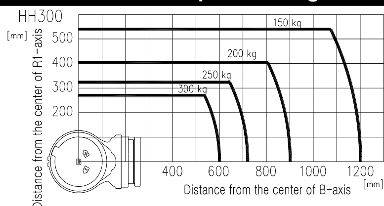
Wrist-axis torque line diagram
