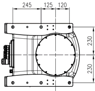
View C: Application cable connection part
