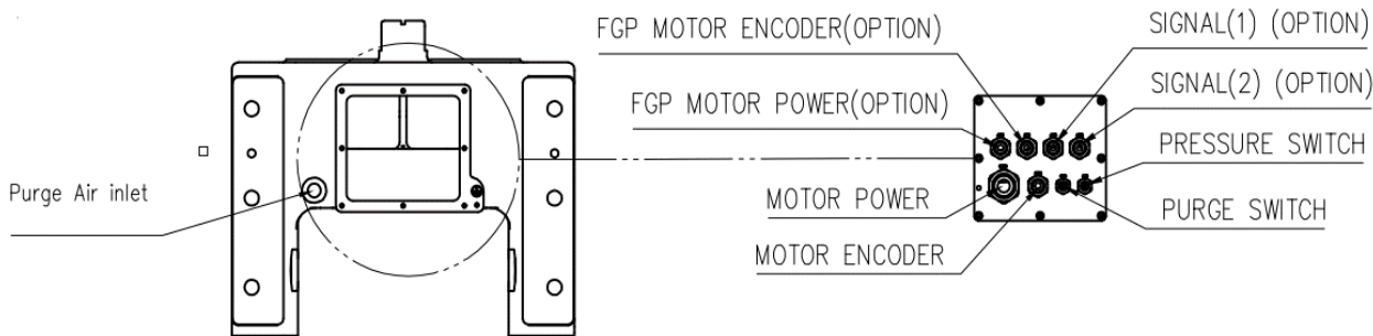
View C: Application cable connection part
