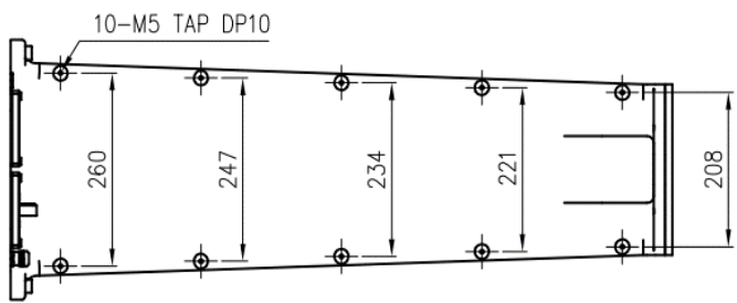
VIEW D: Details of the application ancillary part attachment
