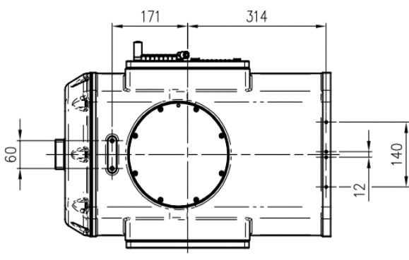
View C: Application cable connection part
