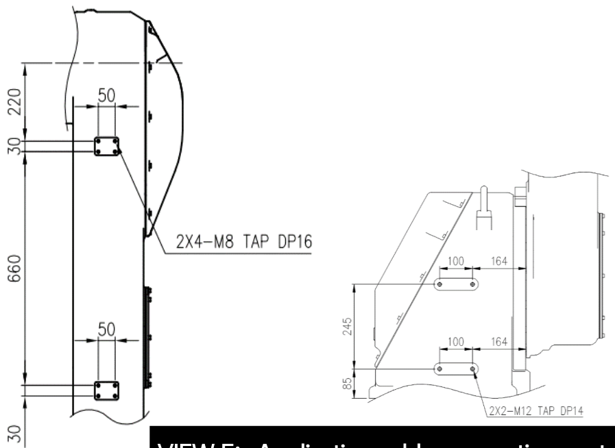
VIEW E: Application cable connection part
