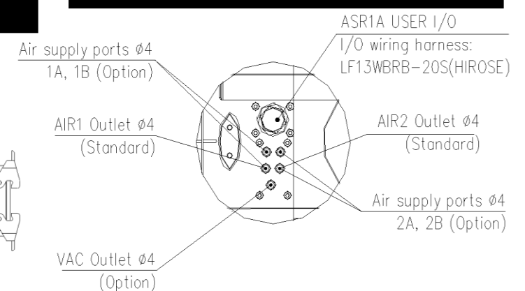
View D: Application cable connection
