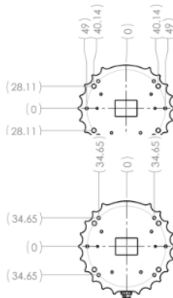
M6 Thread Pattern
