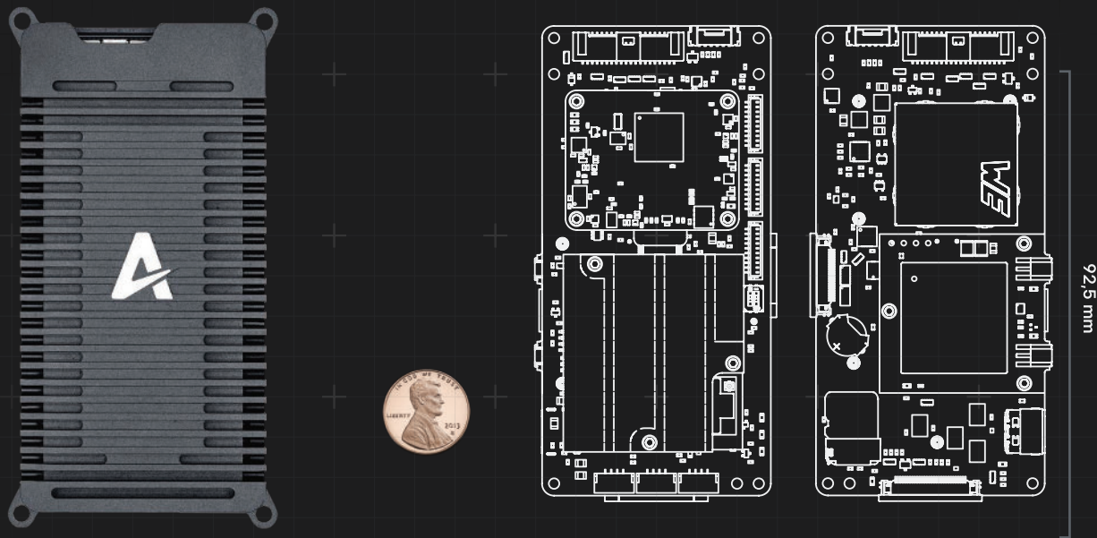
Enclosure dimensions: 110 × 58 × 22.2 mm, weight: approx. 159 g
